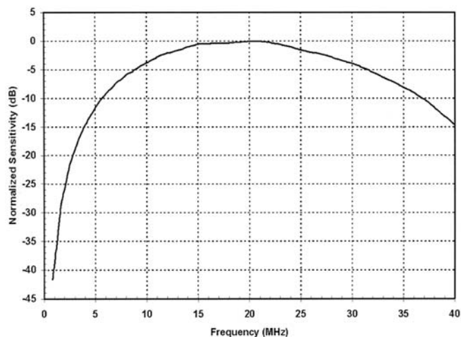
Fig. 2. Combined normalized frequency response of a 0.5-mm diameter coplanar-shielded membrane hydrophone and wideband focused PVDF (source f number, 20).
