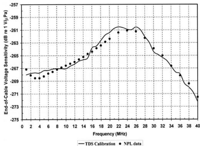
Fig. 3. Frequency response of a 0.5-mm diameter bilaminar PVDF membrane hydrophone. \cdot = NPL data; — = this work (continuous TDS calibration).
