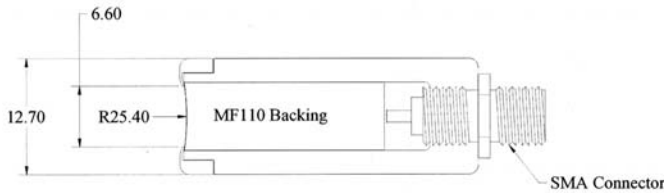
Fig. 1. Schematic construction of the focused polymer source with focal number 4. Two similar sources with f numbers 10 and 20 also were used (dimensions in mm).
