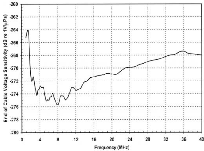
Fig. 4. Frequency response of a 150- \mu effective diameter Specialty Engineering Associates needle PVDF hydrophone with a built-in preamplifier.
