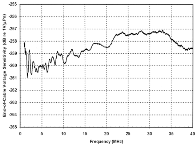
Fig. 5. Frequency response of a new 130- \mu effective diameter "Golden Lipstick" hydrophone (Specialty Engineering Associates, Soquel, CA) as measured using focused PVDF source ( f_n = 20 ).
